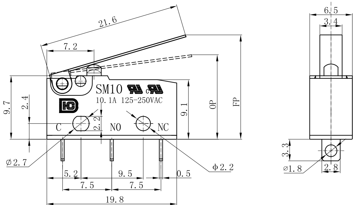
SCHEMATIC
